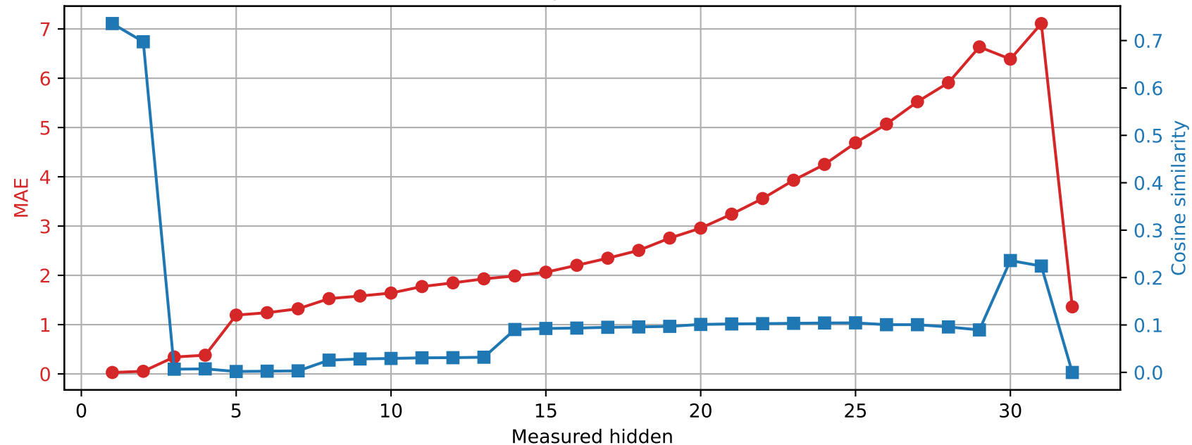
Phi-3-mini-4k-instruct | Prompt 2 Spared layer 10 | Unquantized vs hybrid
