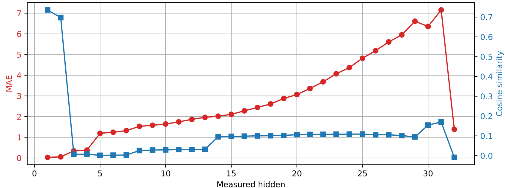
Phi-3-mini-4k-instruct | Prompt 2 Spared layer 26 | Unquantized vs hybrid
