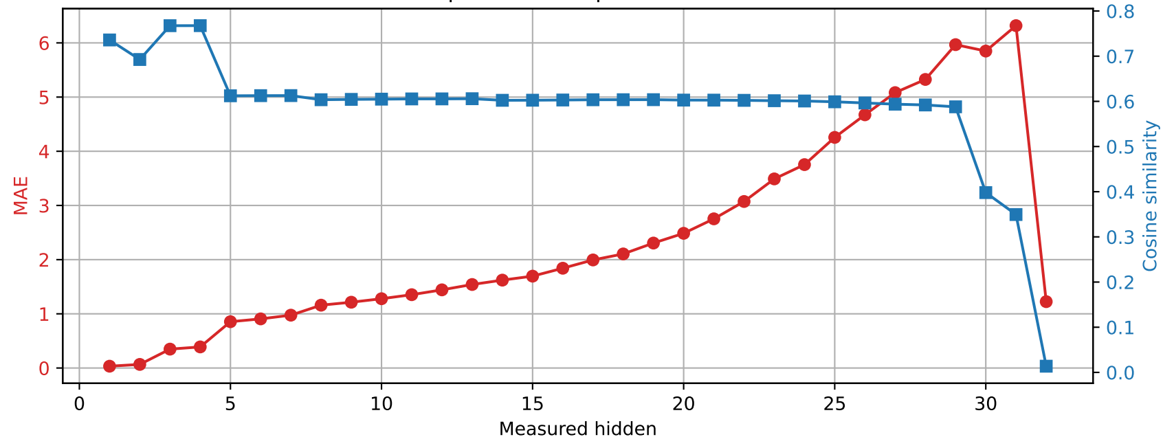
Phi-3-mini-4k-instruct | Prompt 3 Unquantized vs quantized int4
