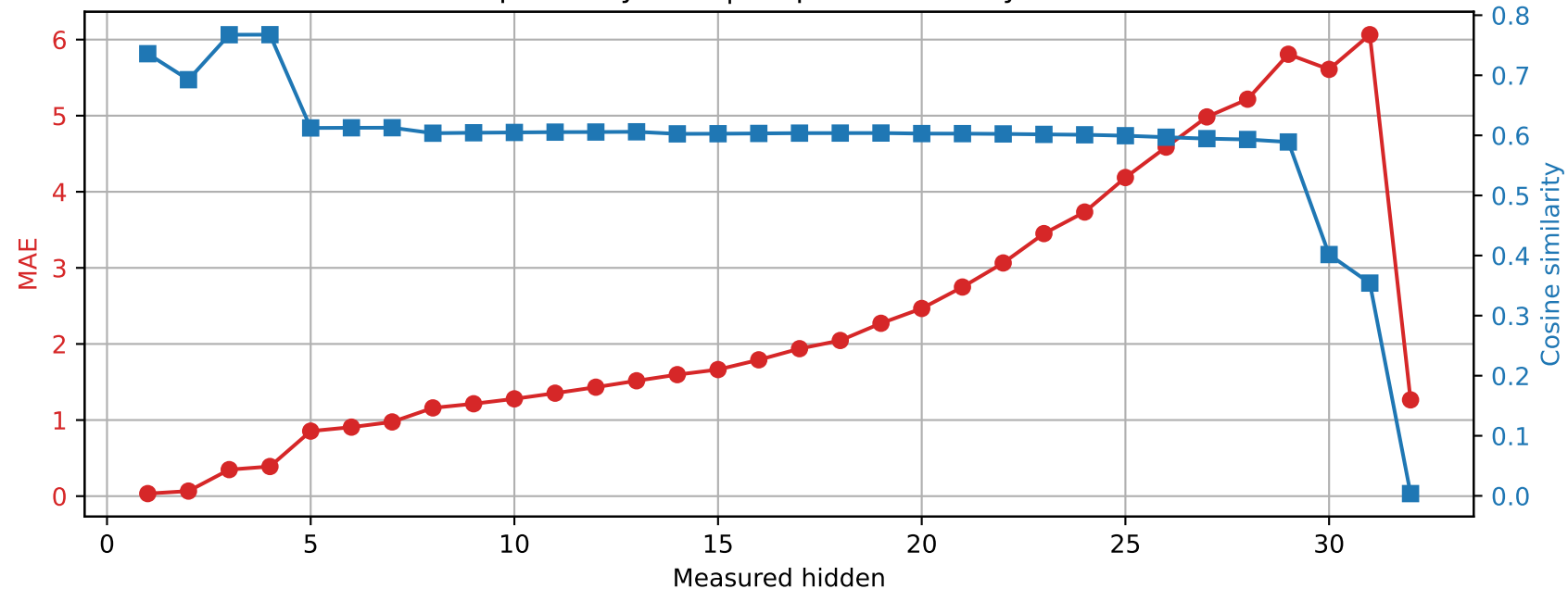
Phi-3-mini-4k-instruct | Prompt 3 Spared layer 11 | Unquantized vs hybrid
