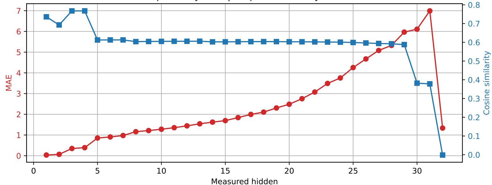
Phi-3-mini-4k-instruct | Prompt 3 Spared layer 29 | Unquantized vs hybrid
