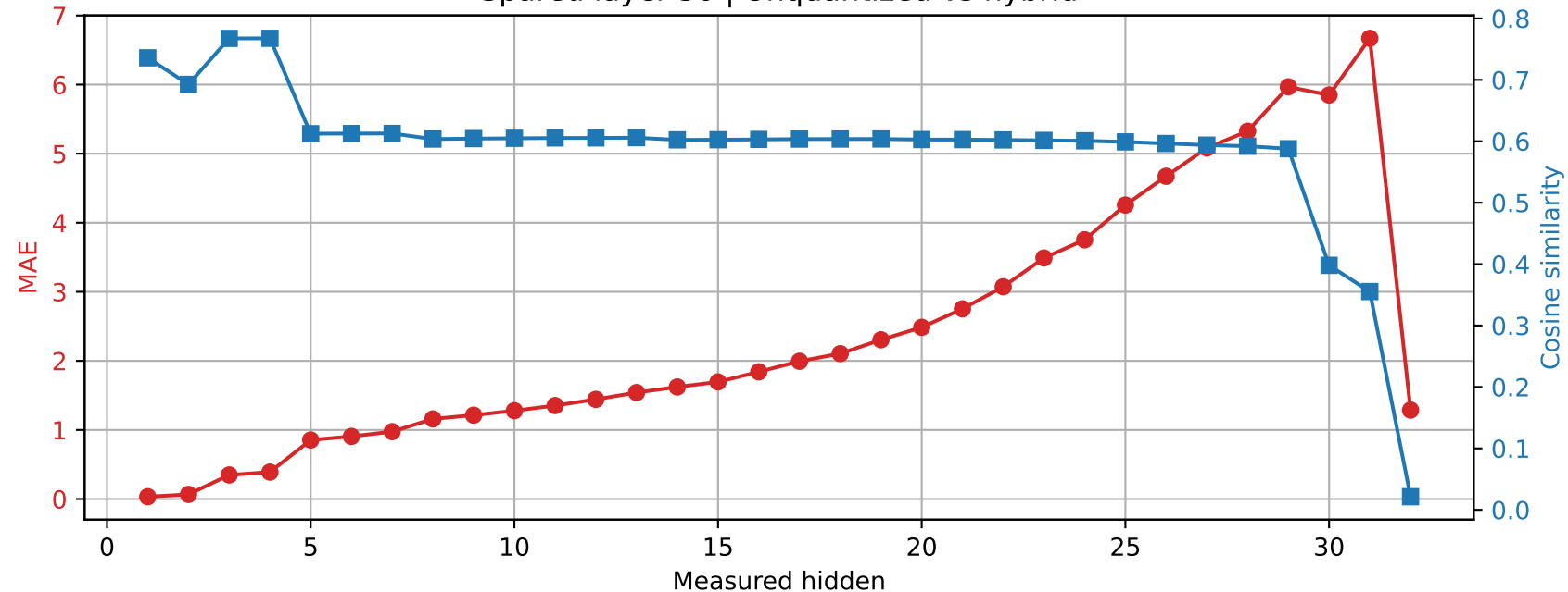
Phi-3-mini-4k-instruct | Prompt 3 Spared layer 30 | Unquantized vs hybrid
