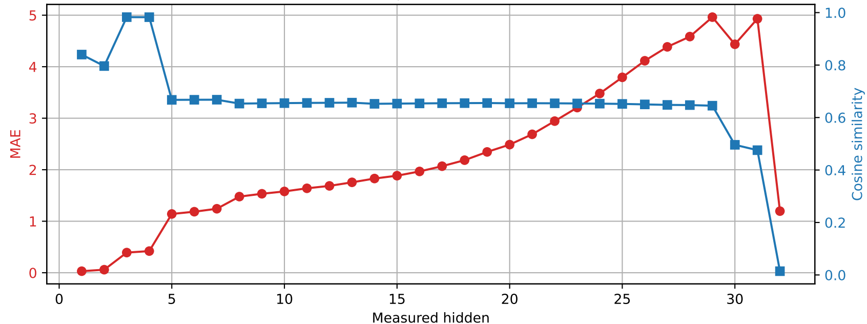
Phi-3-mini-4k-instruct | Prompt 4 Spared layer 5 | Unquantized vs hybrid
