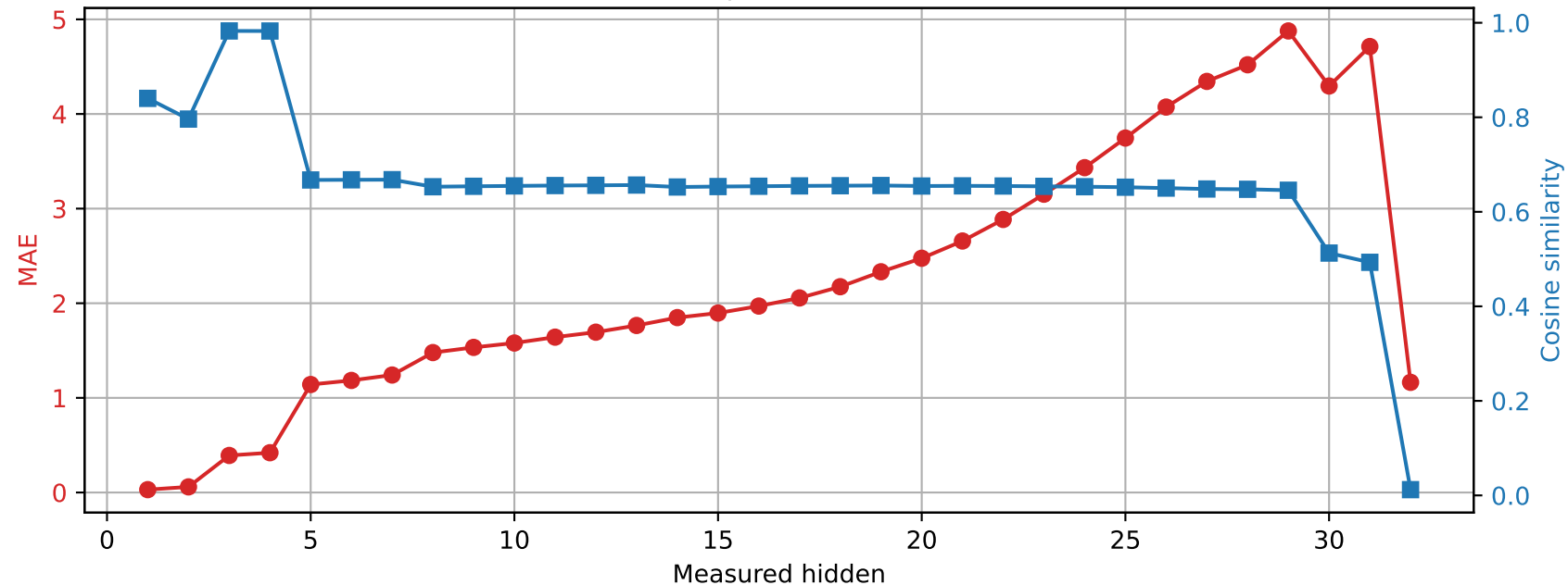
Phi-3-mini-4k-instruct | Prompt 4 Spared layer 13 | Unquantized vs hybrid
