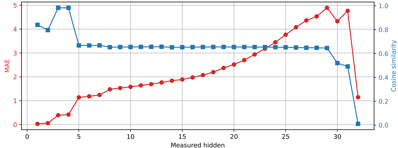
Phi-3-mini-4k-instruct | Prompt 4 Spared layer 22 | Unquantized vs hybrid
