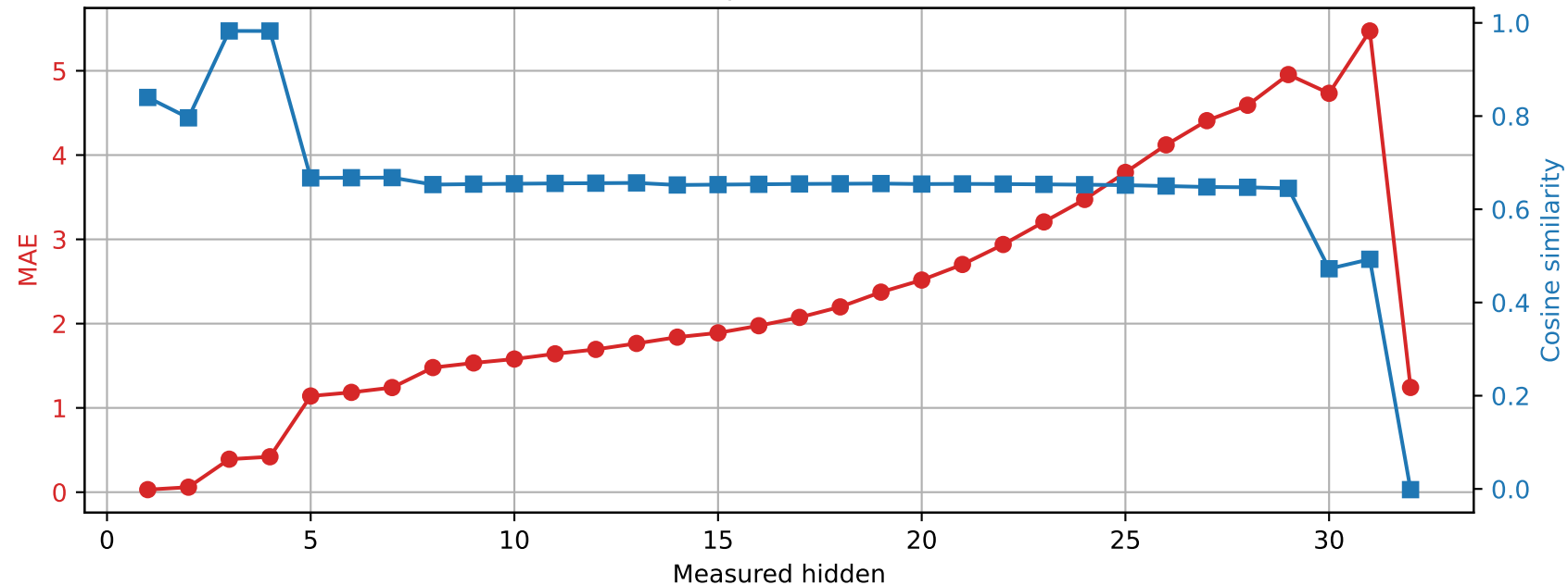
Phi-3-mini-4k-instruct | Prompt 4 Spared layer 29 | Unquantized vs hybrid
