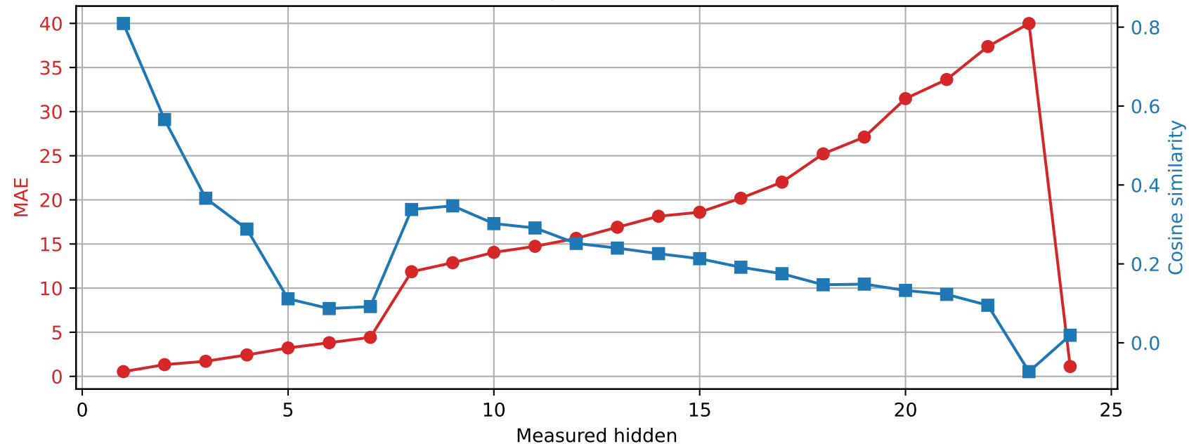
SmolLM2-1.7B-Instruct | Prompt 0 Spared layer 7 | Unquantized vs hybrid
