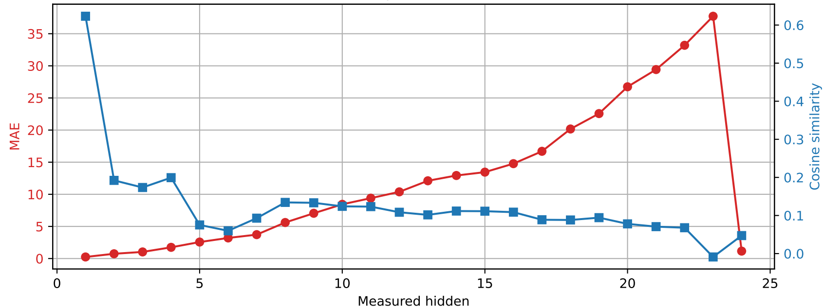
SmolLM2-1.7B-Instruct | Prompt 1 Spared layer 13 | Unquantized vs hybrid
