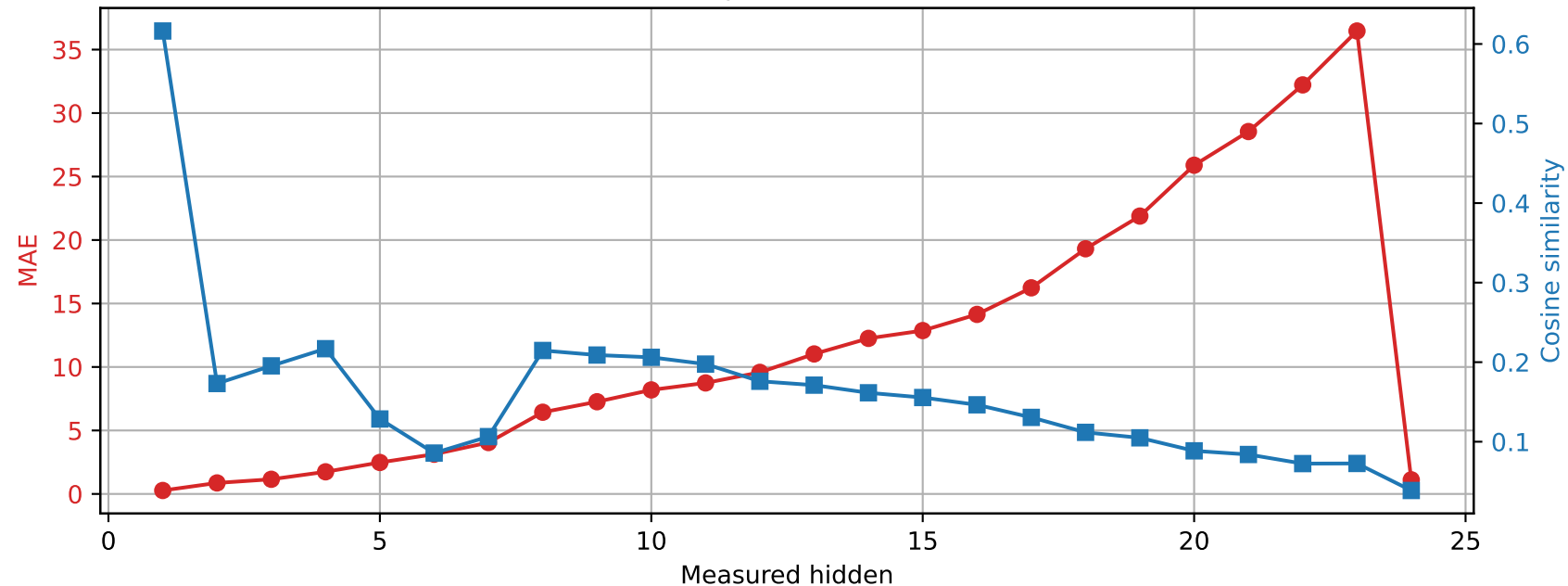
SmolLM2-1.7B-Instruct | Prompt 2 Spared layer 6 | Unquantized vs hybrid
