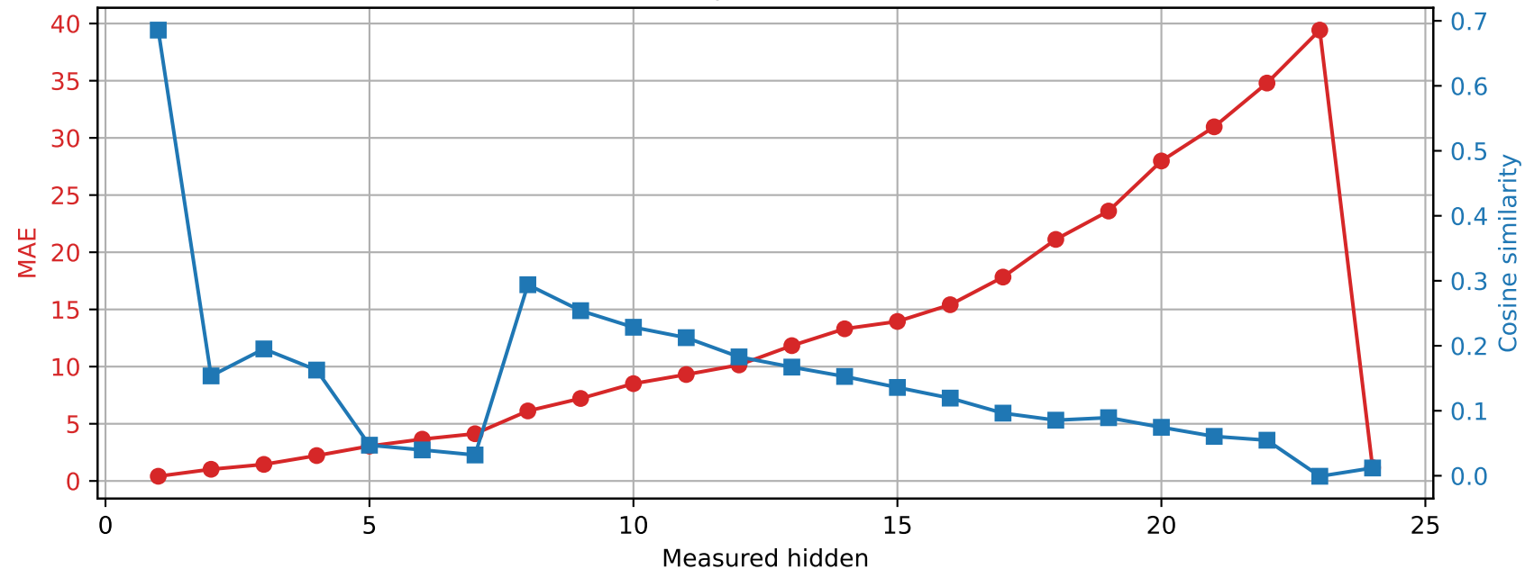
SmolLM2-1.7B-Instruct | Prompt 3 Spared layer 16 | Unquantized vs hybrid
