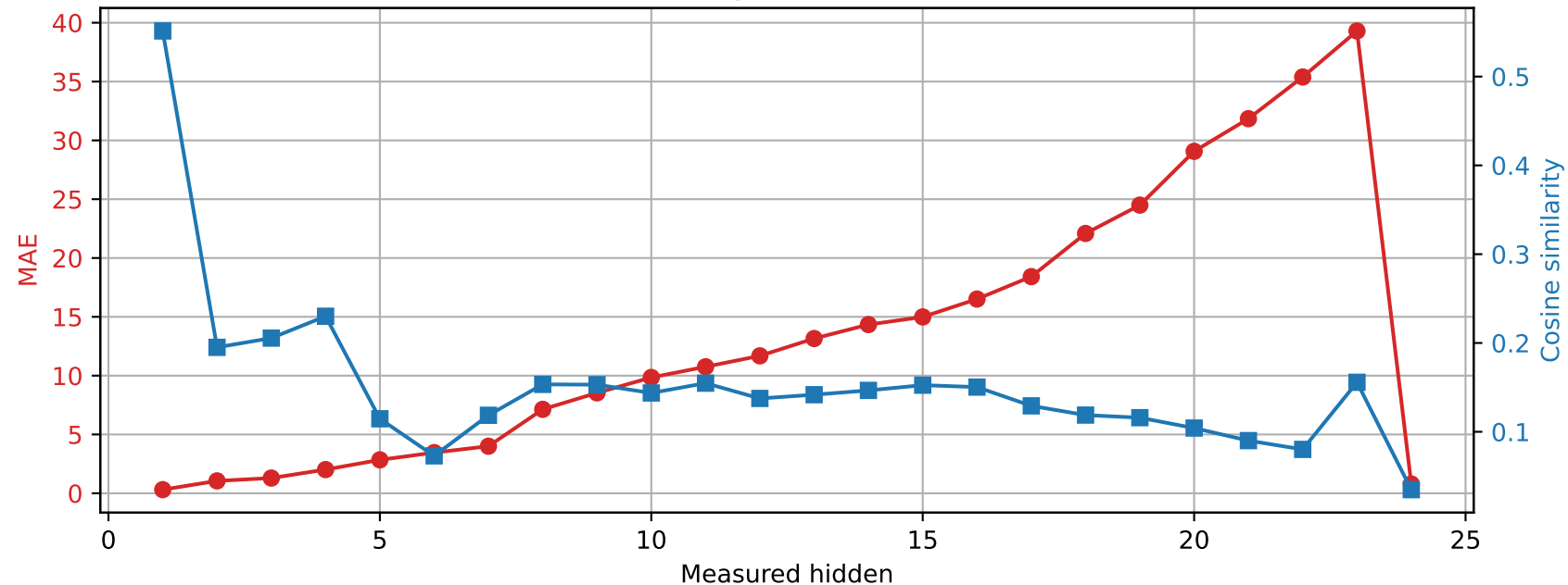
SmolLM2-1.7B-Instruct | Prompt 4 Spared layer 21 | Unquantized vs hybrid
