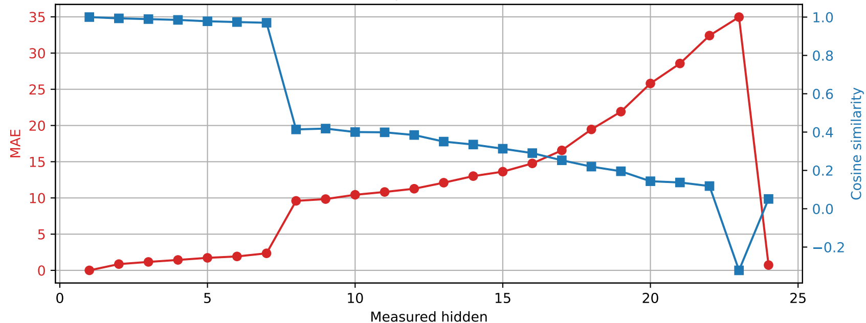
SmolLM2-1.7B-Instruct | Prompt 0 Spared layer 0 | Unquantized vs hybrid
