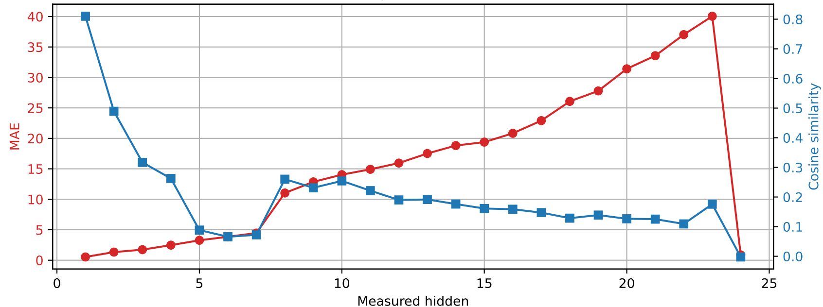
SmolLM2-1.7B-Instruct | Prompt 0 Spared layer 8 | Unquantized vs hybrid
