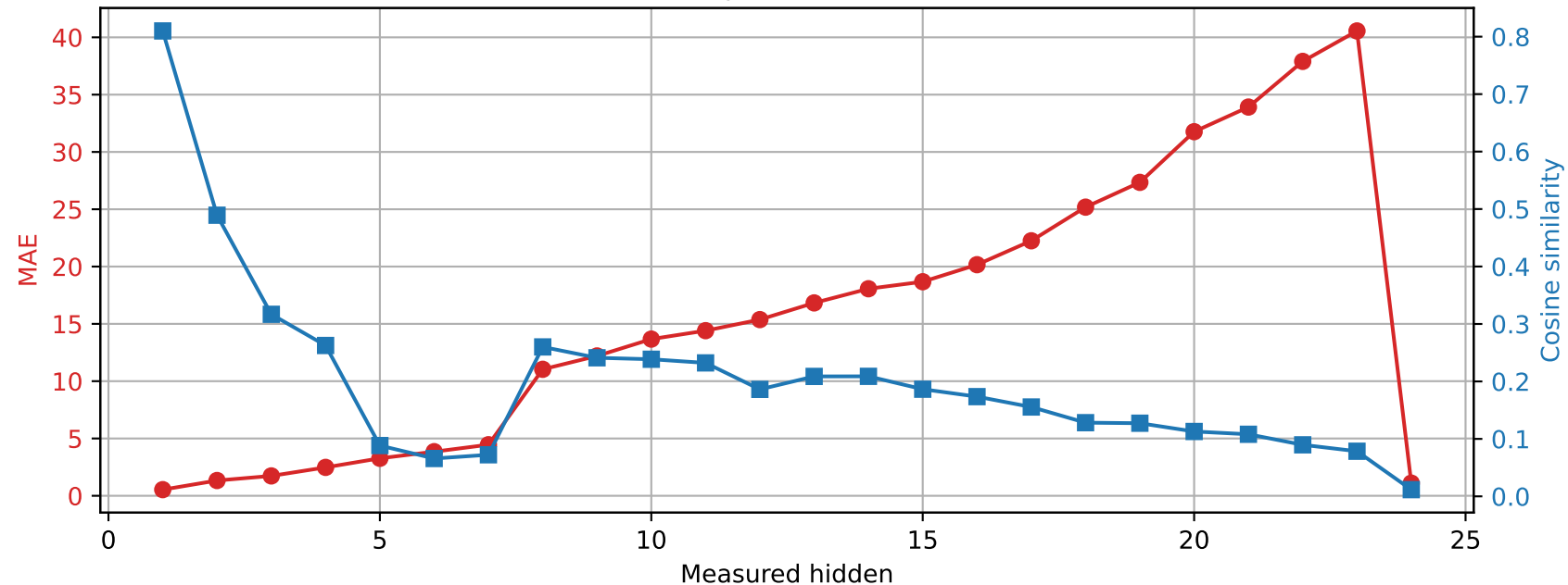
SmolLM2-1.7B-Instruct | Prompt 0 Spared layer 9 | Unquantized vs hybrid
