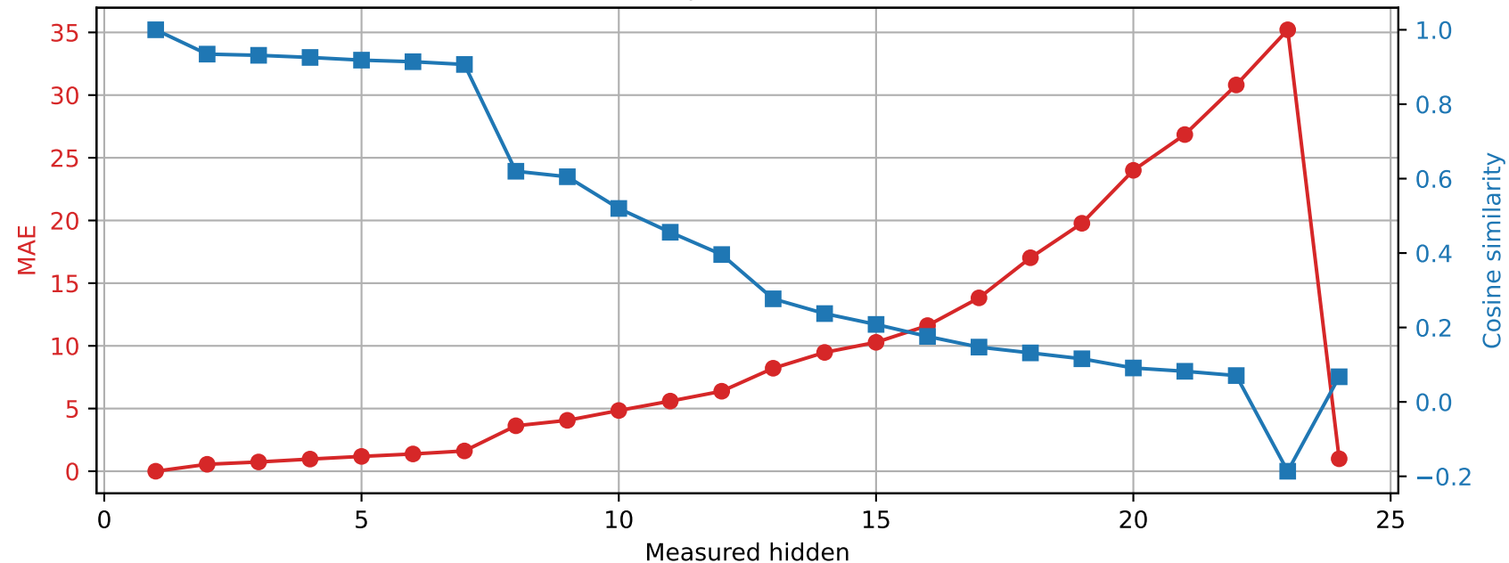
SmolLM2-1.7B-Instruct | Prompt 1 Spared layer 0 | Unquantized vs hybrid
