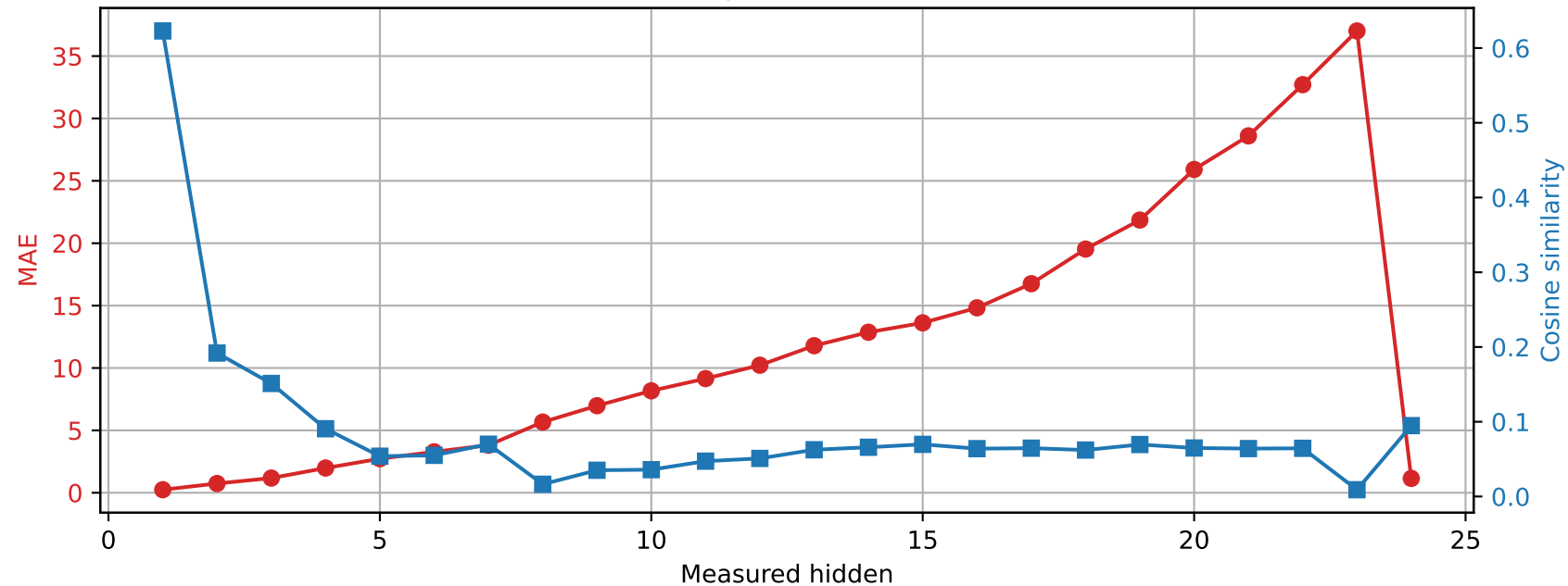
SmolLM2-1.7B-Instruct | Prompt 1 Spared layer 2 | Unquantized vs hybrid
