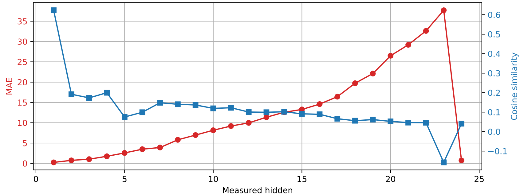
SmolLM2-1.7B-Instruct | Prompt 1 Spared layer 5 | Unquantized vs hybrid
