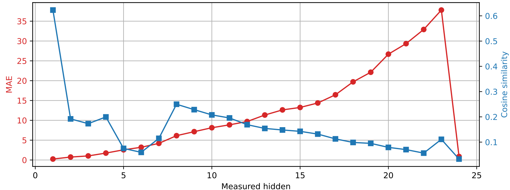
SmolLM2-1.7B-Instruct | Prompt 1 Spared layer 6 | Unquantized vs hybrid
