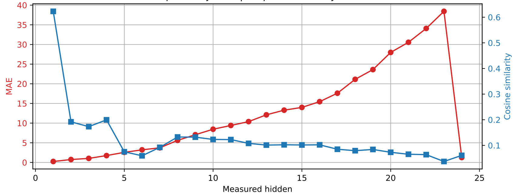
SmolLM2-1.7B-Instruct | Prompt 1 Spared layer 23 | Unquantized vs hybrid
