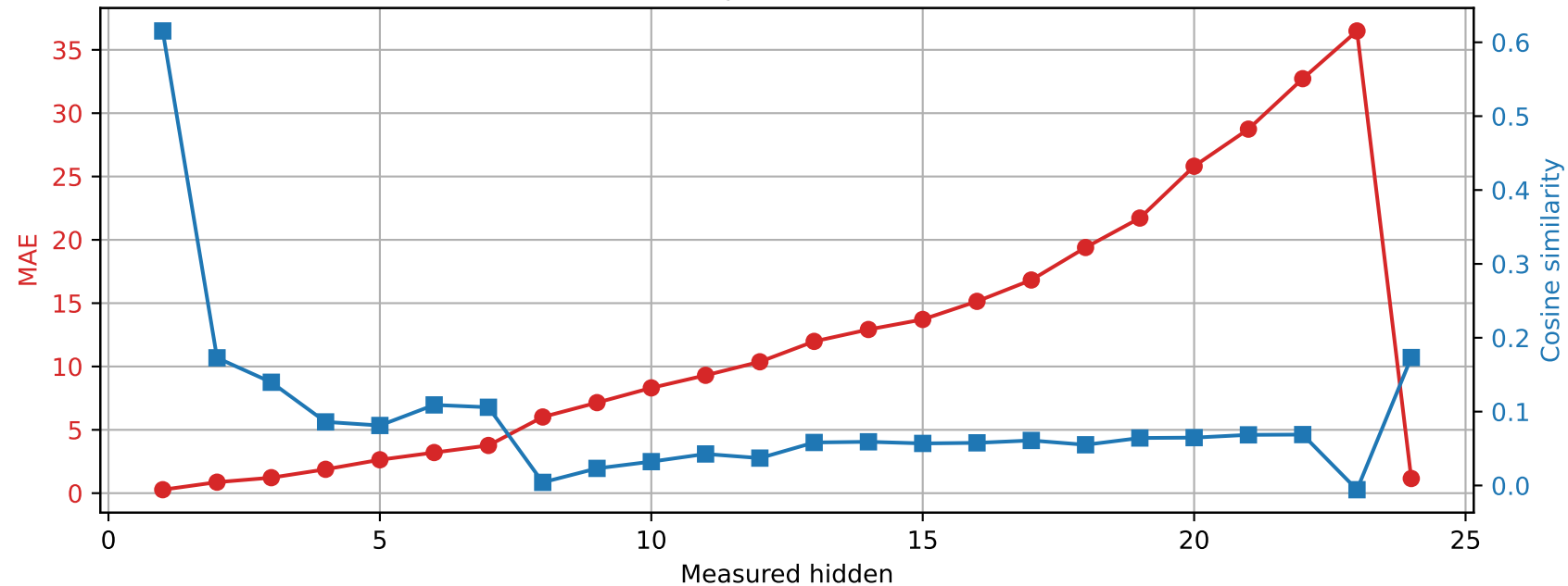
SmolLM2-1.7B-Instruct | Prompt 2 Spared layer 2 | Unquantized vs hybrid
