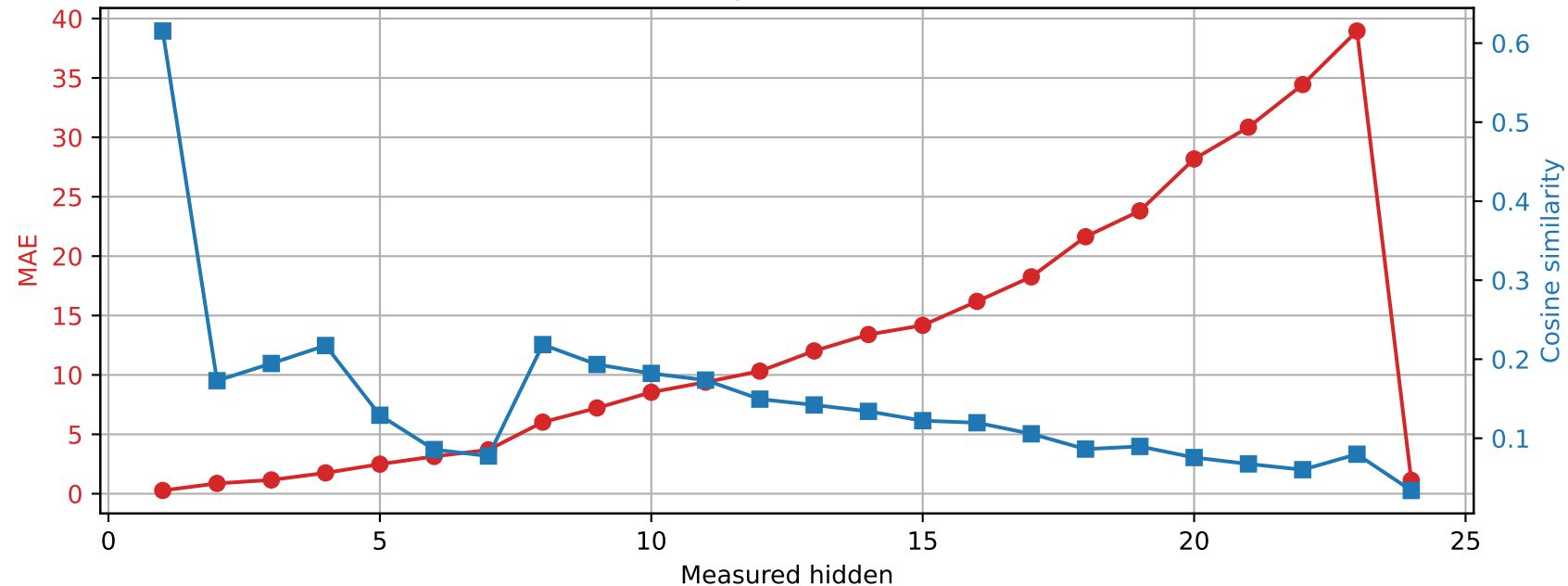
SmolLM2-1.7B-Instruct | Prompt 2 Spared layer 15 | Unquantized vs hybrid
