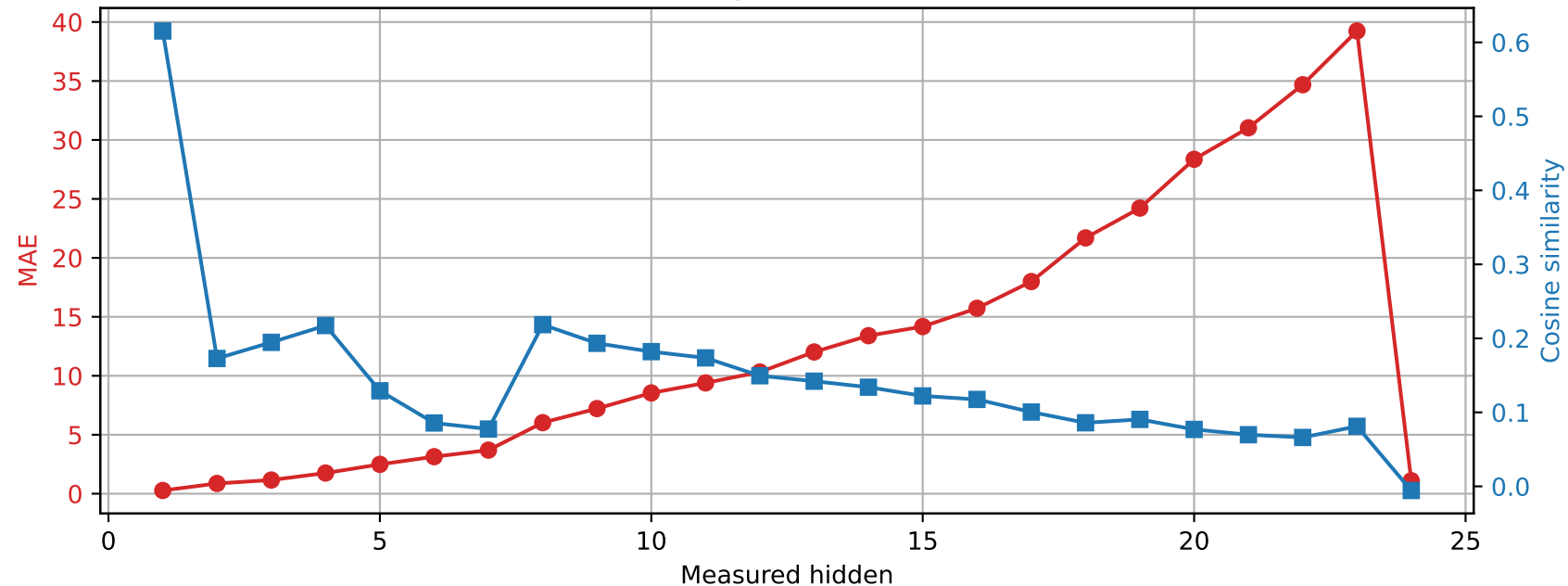
SmolLM2-1.7B-Instruct | Prompt 2 Spared layer 23 | Unquantized vs hybrid
