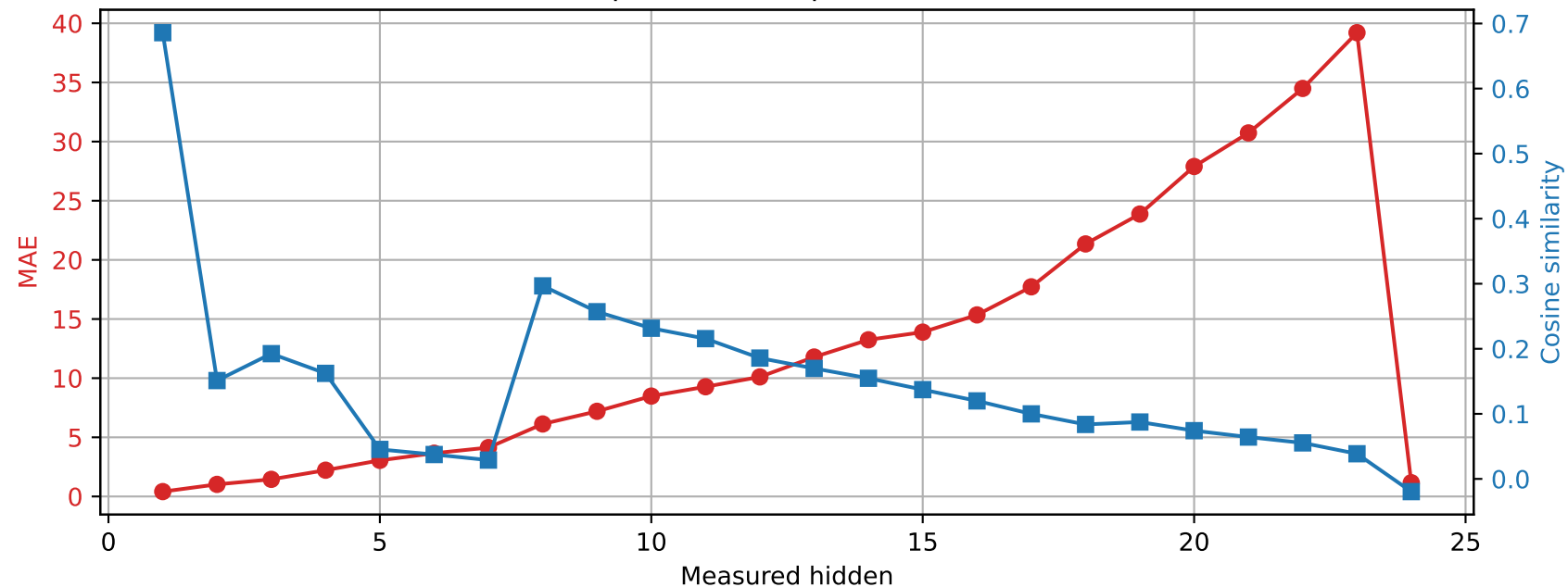
SmolLM2-1.7B-Instruct | Prompt 3 Unquantized vs quantized int4
