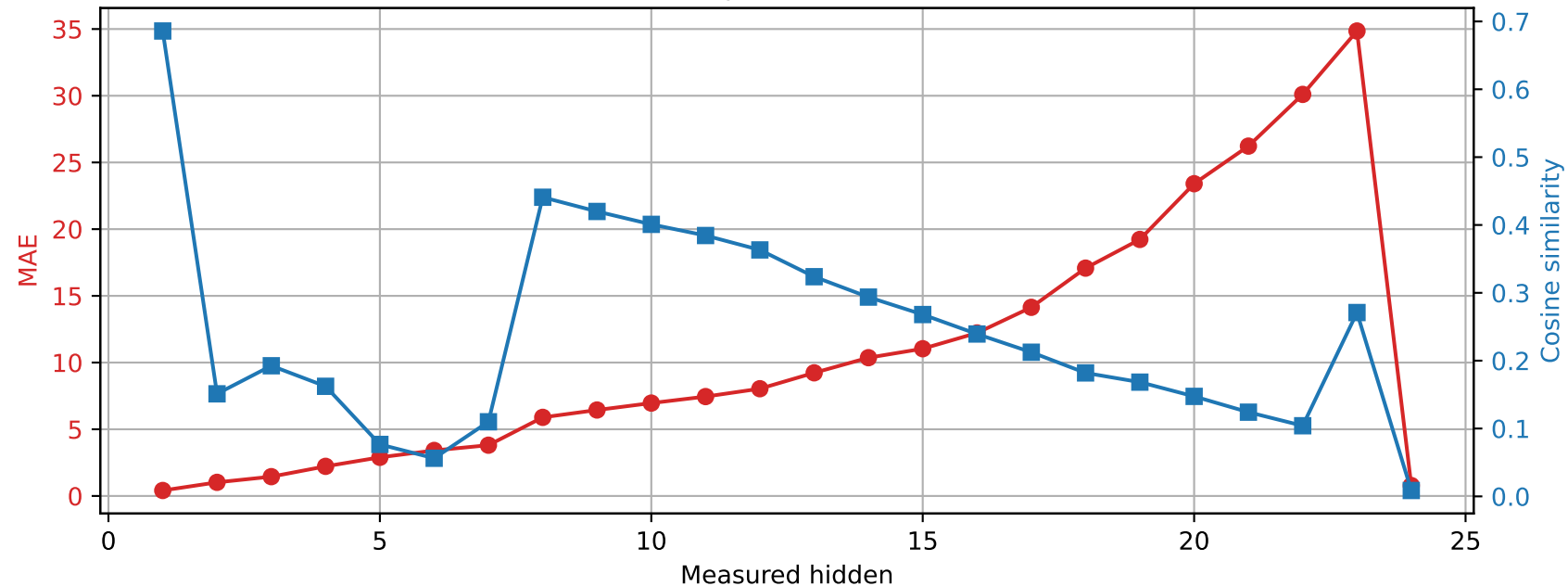
SmolLM2-1.7B-Instruct | Prompt 3 Spared layer 4 | Unquantized vs hybrid
