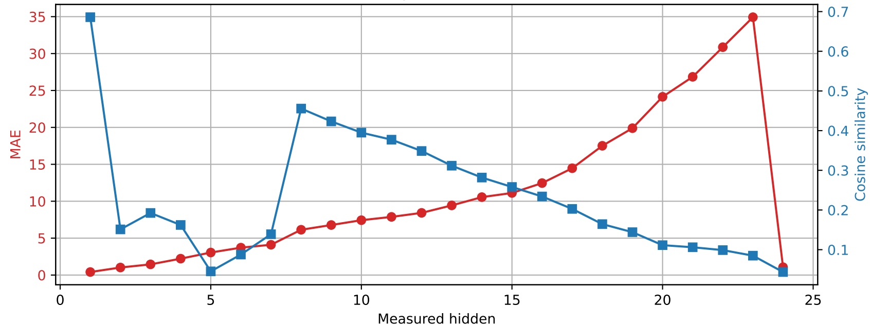
SmolLM2-1.7B-Instruct | Prompt 3 Spared layer 5 | Unquantized vs hybrid
