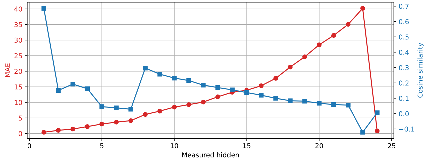
SmolLM2-1.7B-Instruct | Prompt 3 Spared layer 18 | Unquantized vs hybrid
