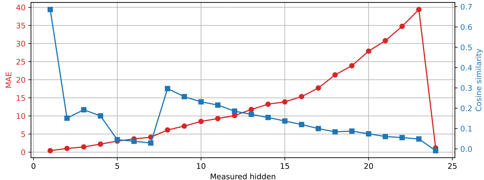
SmolLM2-1.7B-Instruct | Prompt 3 Spared layer 20 | Unquantized vs hybrid
