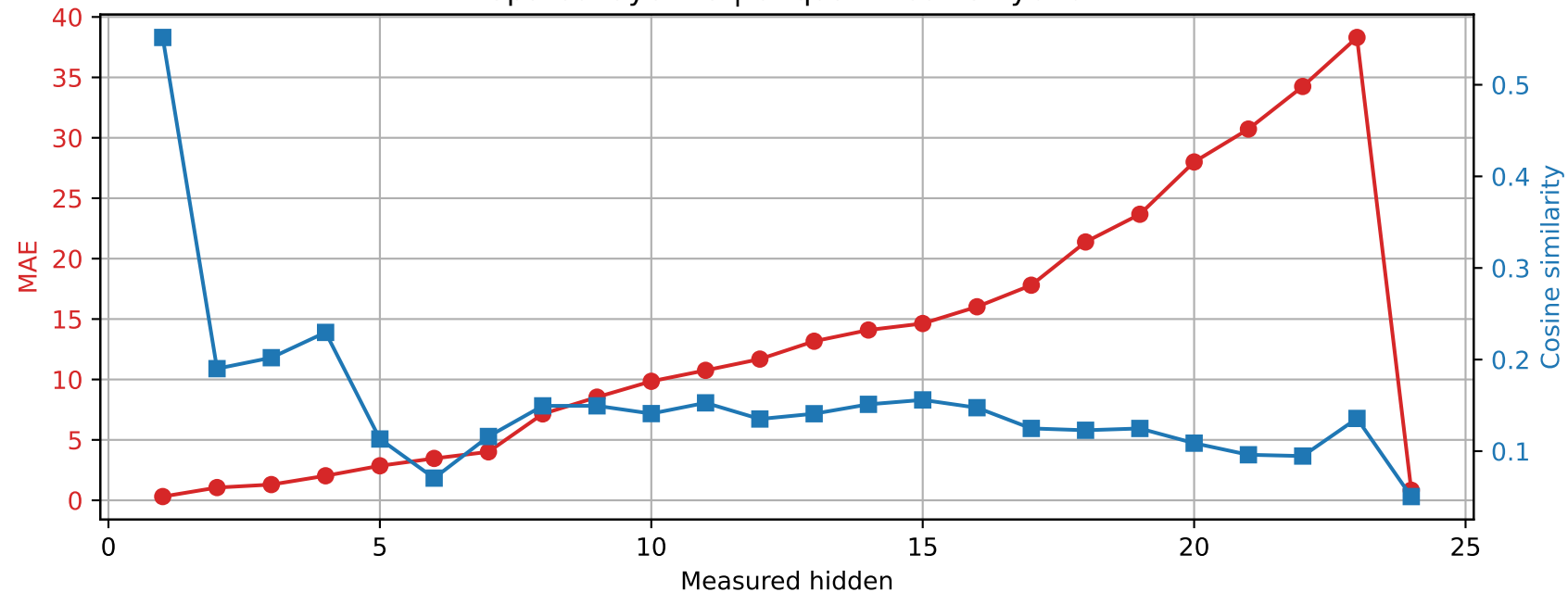
SmolLM2-1.7B-Instruct | Prompt 4 Spared layer 13 | Unquantized vs hybrid
