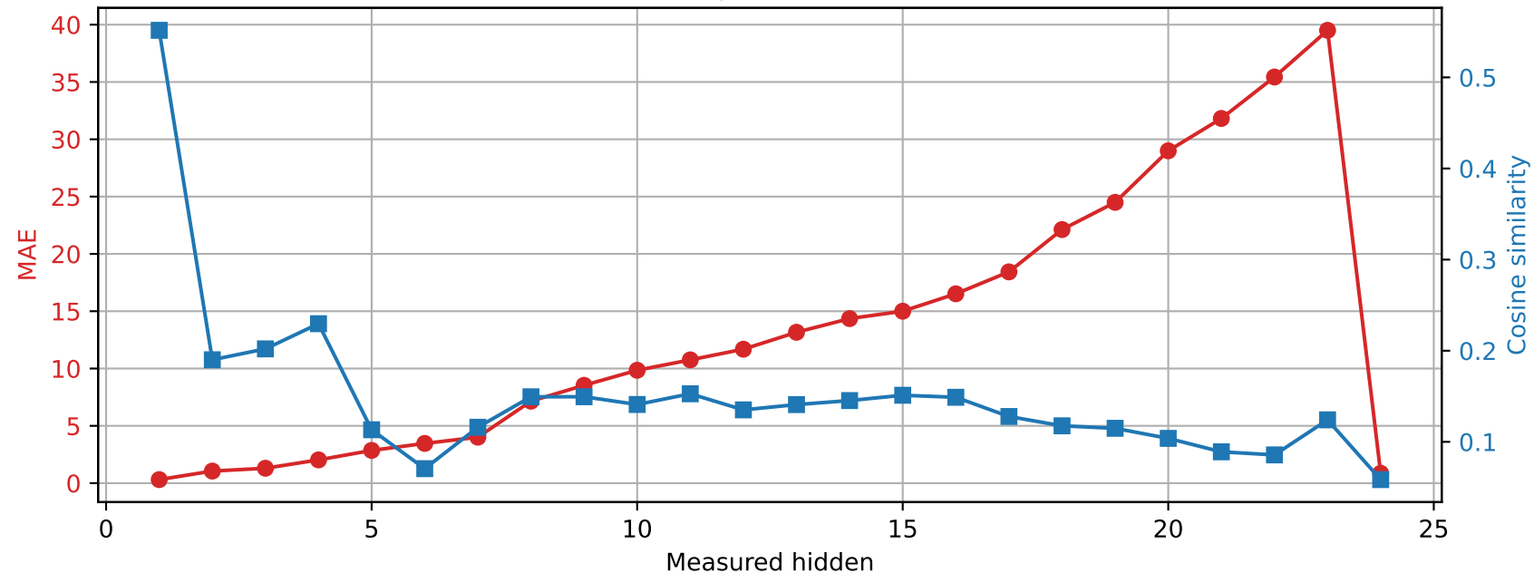
SmolLM2-1.7B-Instruct | Prompt 4 Spared layer 22 | Unquantized vs hybrid
