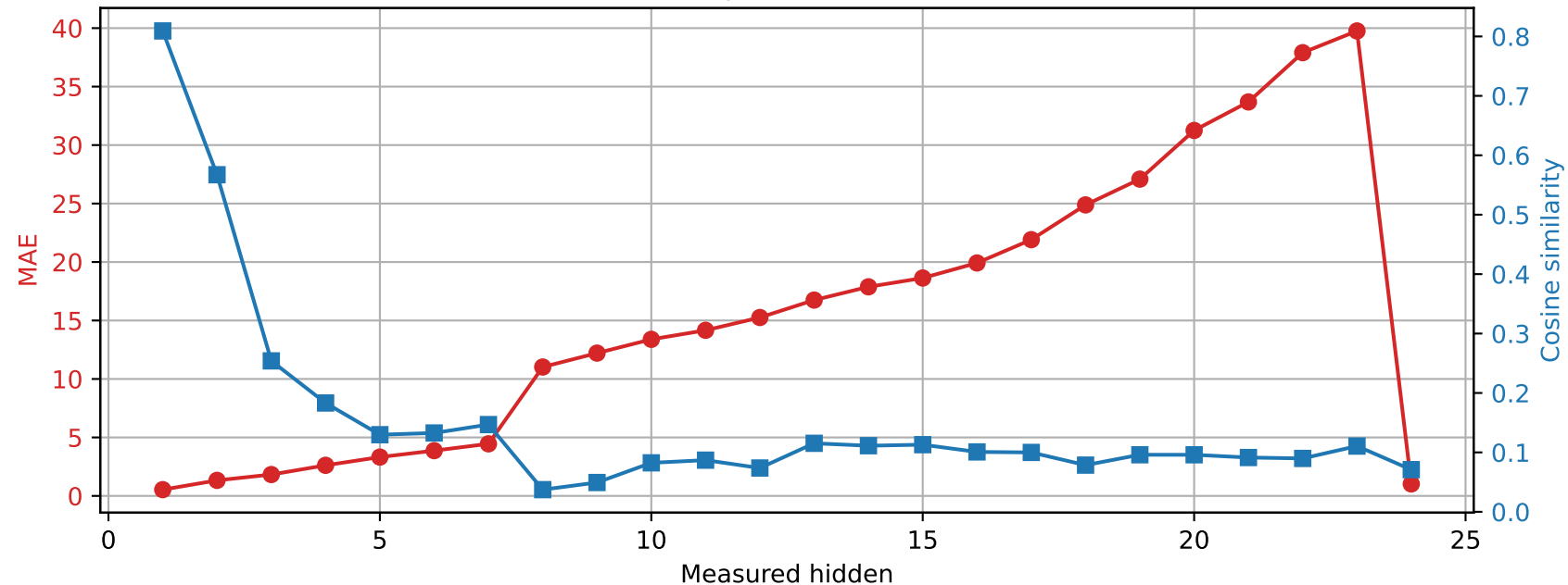
SmolLM2-1.7B-Instruct | Prompt 0 Spared layer 2 | Unquantized vs hybrid
