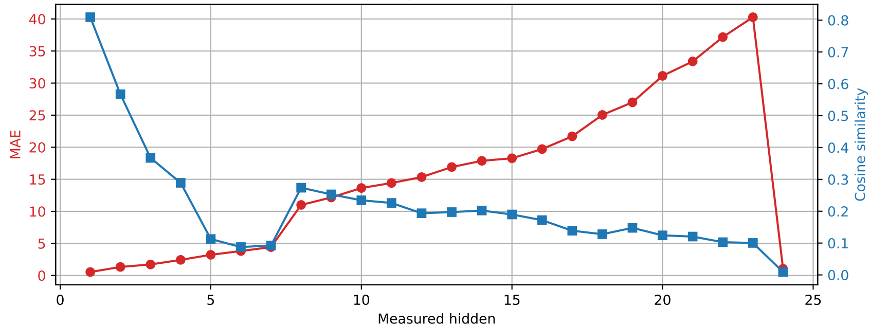
SmolLM2-1.7B-Instruct | Prompt 0 Spared layer 13 | Unquantized vs hybrid
