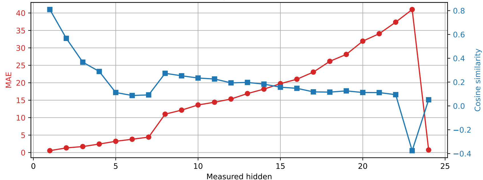
SmolLM2-1.7B-Instruct | Prompt 0 Spared layer 14 | Unquantized vs hybrid
