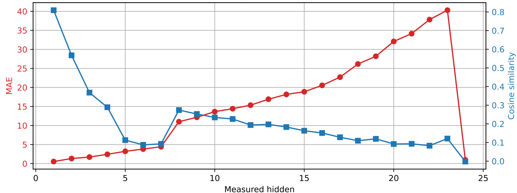
SmolLM2-1.7B-Instruct | Prompt 0 Spared layer 19 | Unquantized vs hybrid
