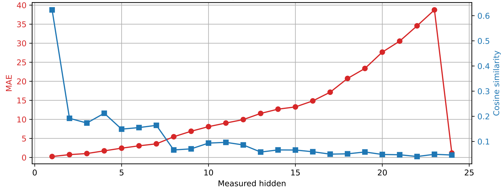
SmolLM2-1.7B-Instruct | Prompt 1 Spared layer 3 | Unquantized vs hybrid
