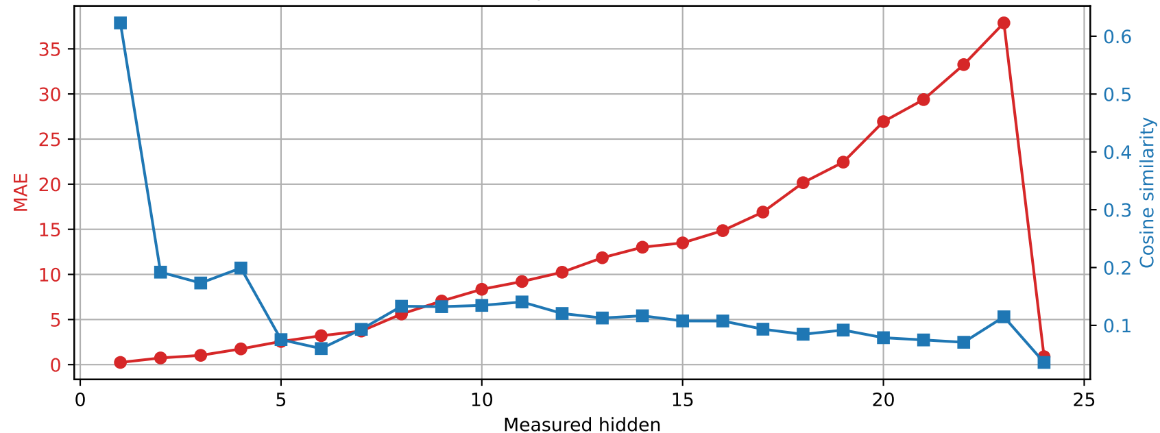
SmolLM2-1.7B-Instruct | Prompt 1 Spared layer 9 | Unquantized vs hybrid
