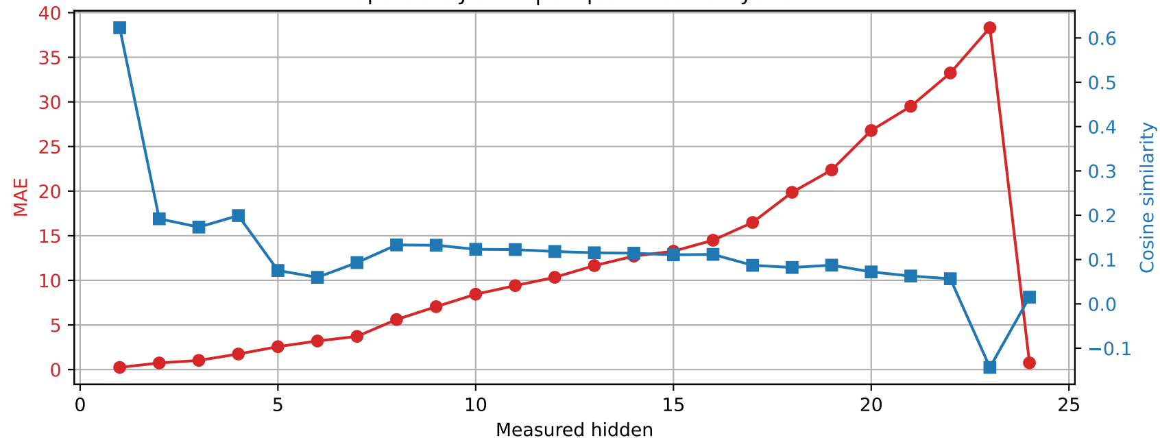
SmolLM2-1.7B-Instruct | Prompt 1 Spared layer 11 | Unquantized vs hybrid
