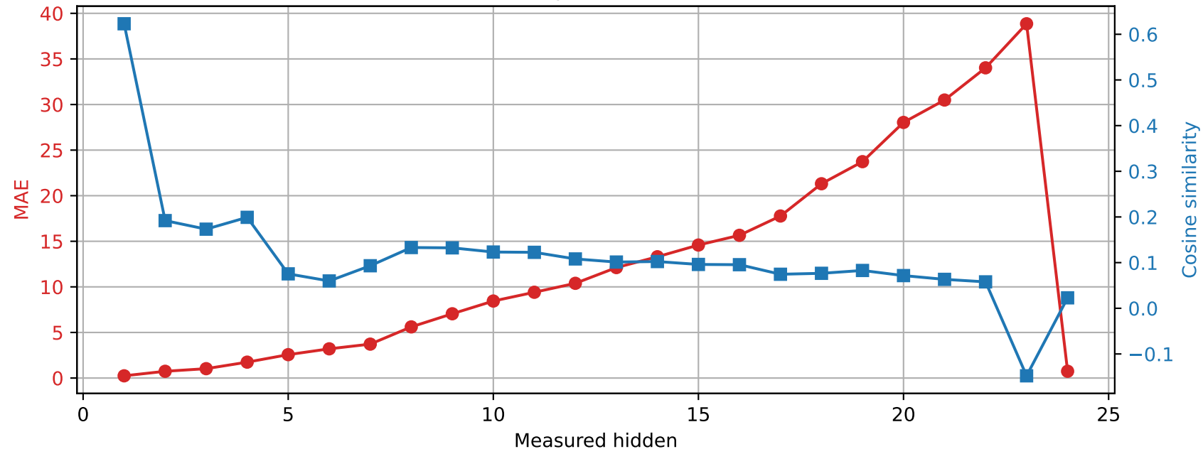
SmolLM2-1.7B-Instruct | Prompt 1 Spared layer 14 | Unquantized vs hybrid
