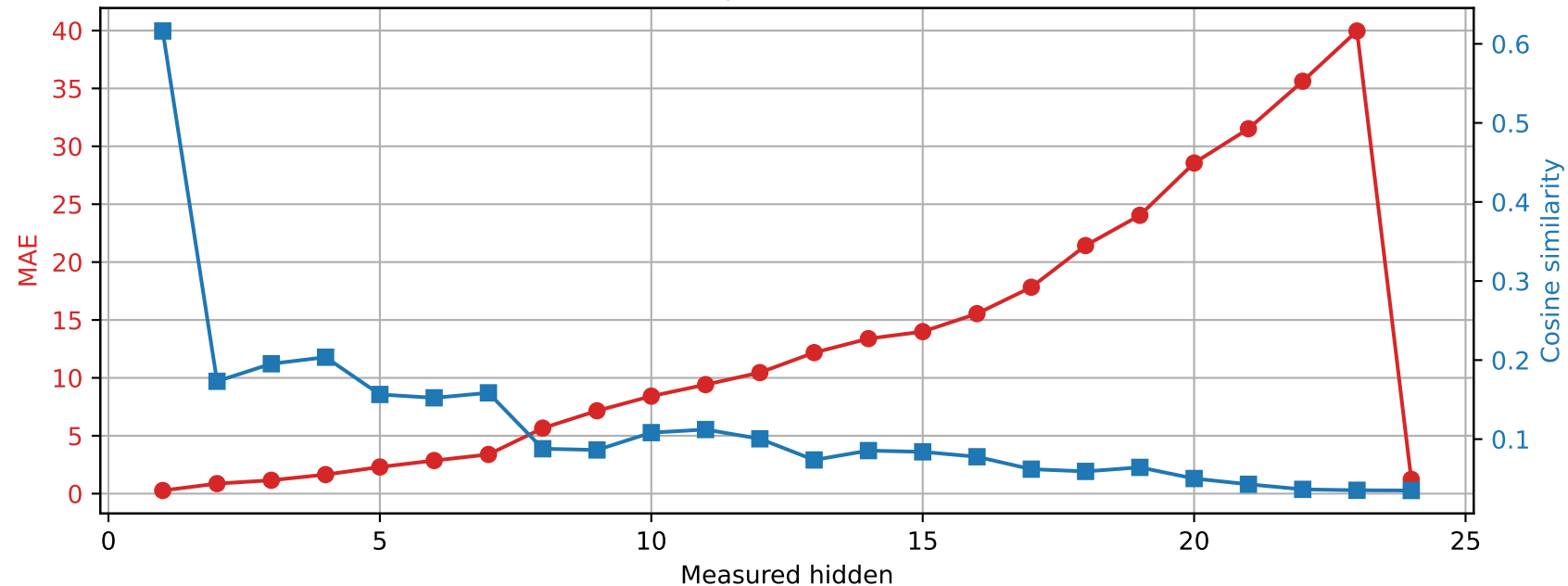
SmolLM2-1.7B-Instruct | Prompt 2 Spared layer 3 | Unquantized vs hybrid
