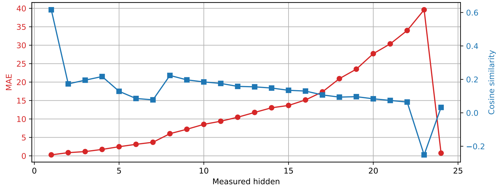
SmolLM2-1.7B-Instruct | Prompt 2 Spared layer 11 | Unquantized vs hybrid
