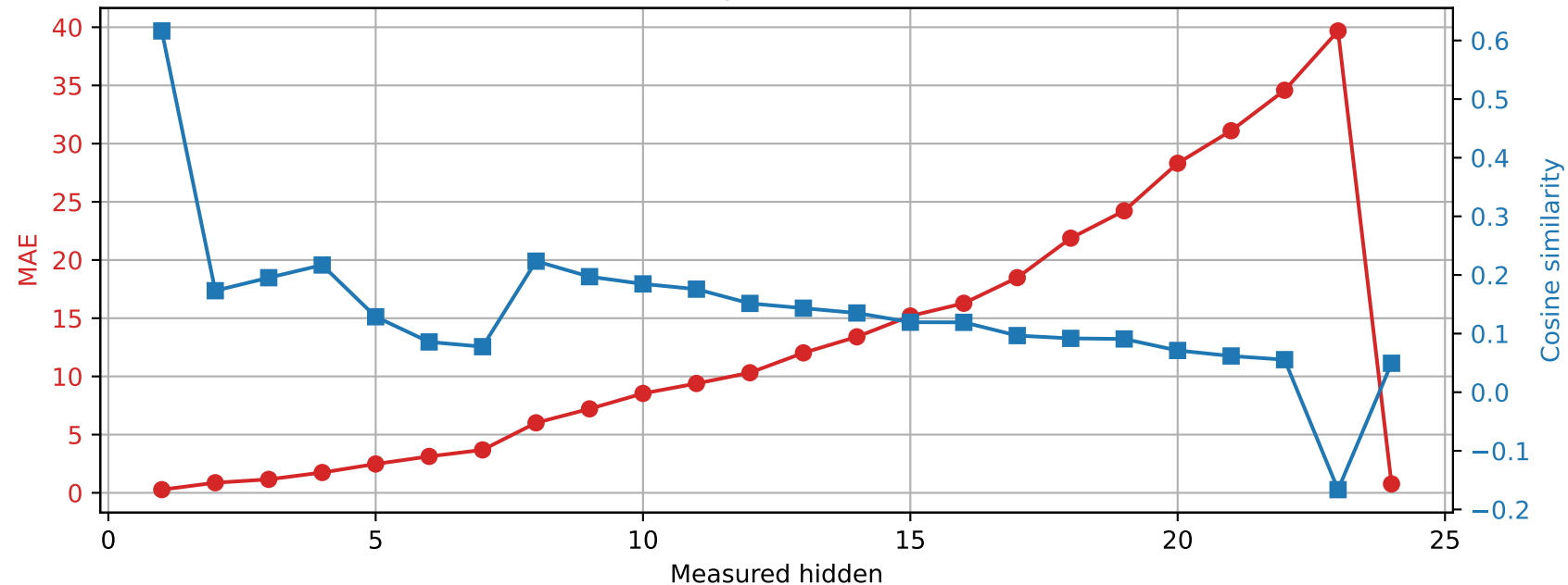
SmolLM2-1.7B-Instruct | Prompt 2 Spared layer 14 | Unquantized vs hybrid
