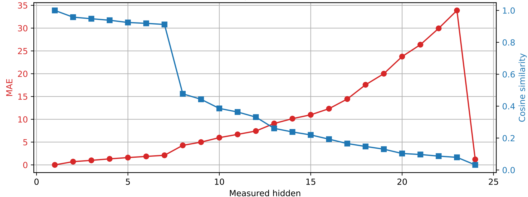
SmolLM2-1.7B-Instruct | Prompt 3 Spared layer 0 | Unquantized vs hybrid
