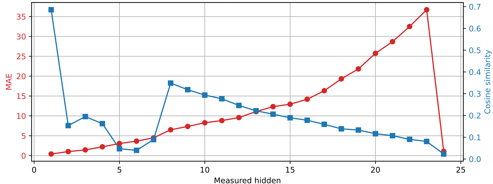
SmolLM2-1.7B-Instruct | Prompt 3 Spared layer 6 | Unquantized vs hybrid
