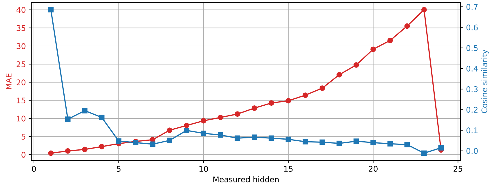
SmolLM2-1.7B-Instruct | Prompt 3 Spared layer 7 | Unquantized vs hybrid
