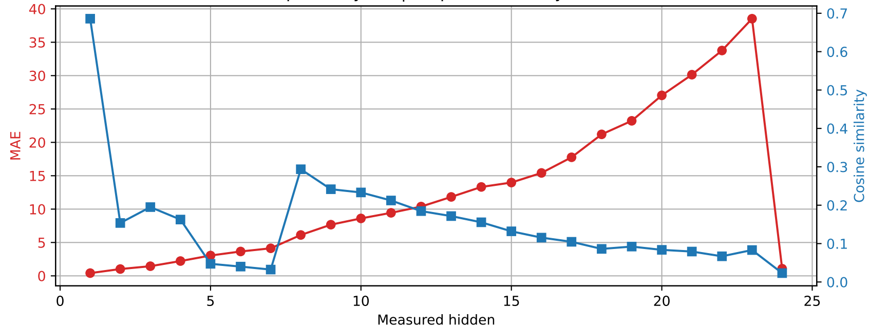
SmolLM2-1.7B-Instruct | Prompt 3 Spared layer 8 | Unquantized vs hybrid
