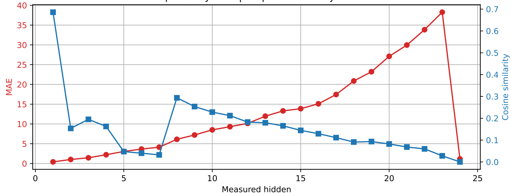
SmolLM2-1.7B-Instruct | Prompt 3 Spared layer 12 | Unquantized vs hybrid
