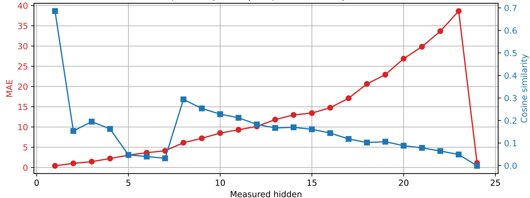
SmolLM2-1.7B-Instruct | Prompt 3 Spared layer 13 | Unquantized vs hybrid
